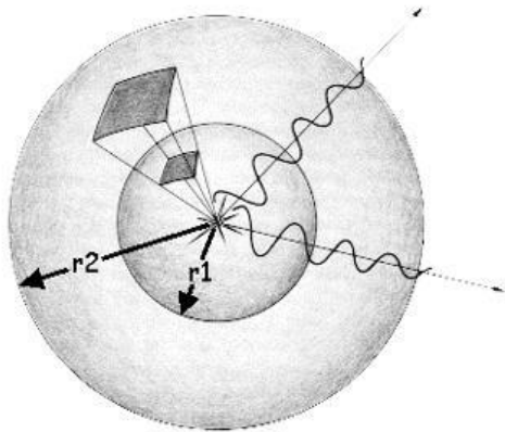
Spherical waves
