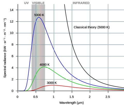
Black-body radiation
